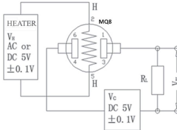
Figure A3 : Circuit interne MQ8
